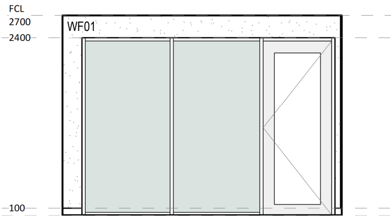
5 ELEVATION DETAIL 60-044 1 : 50
