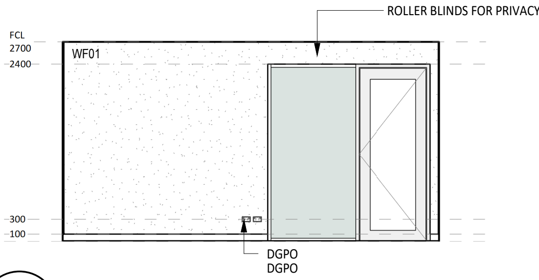
4 ELEVATION DETAIL 60-045 1 : 50
