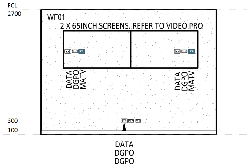
3 ELEVATION DETAIL 60-044 1 : 50
